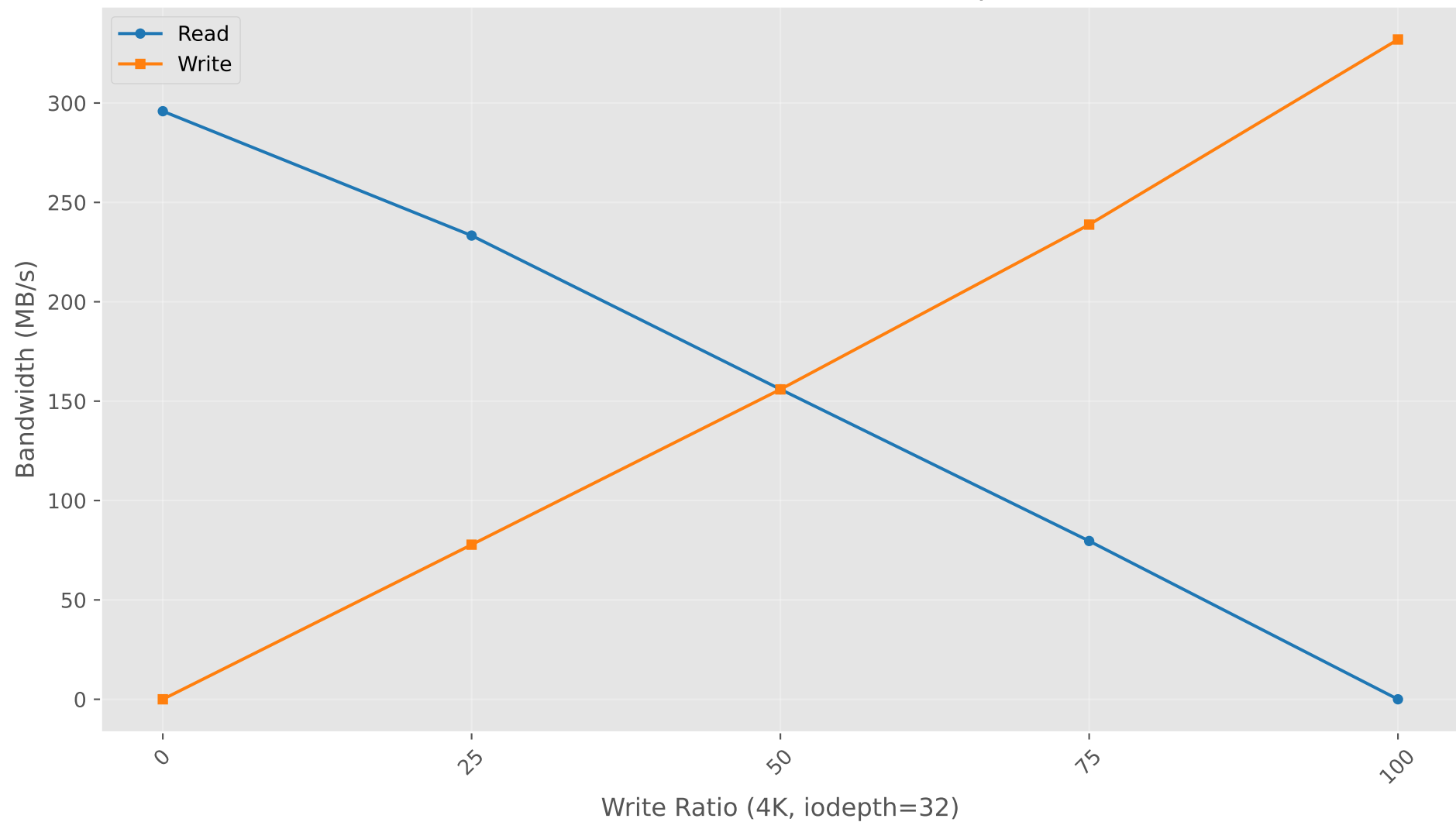
Bandwidth vs Write Ratio (4K, iodepth=32)
